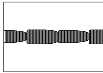
SECAM PB 0.36 Vp-p 20 mV/1 msec/DIV
