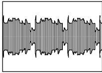
SECAM REC 0.44 Vp-p 10 mV/20 μsec/DIV
