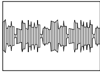
SECAM PB 0.44 Vp-p 20 mV/20 μsec/DIV
